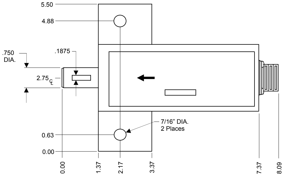
Figure 5.1 Top View
