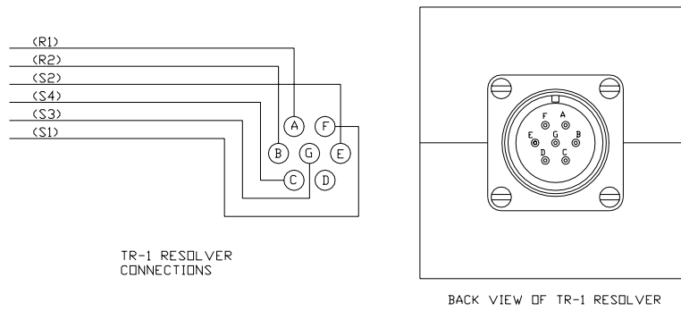
Figure 3.1 TR-1 Electrical connections
