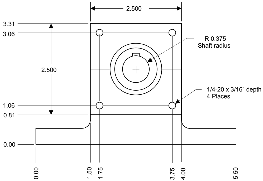
Figure 5.2 Front View
