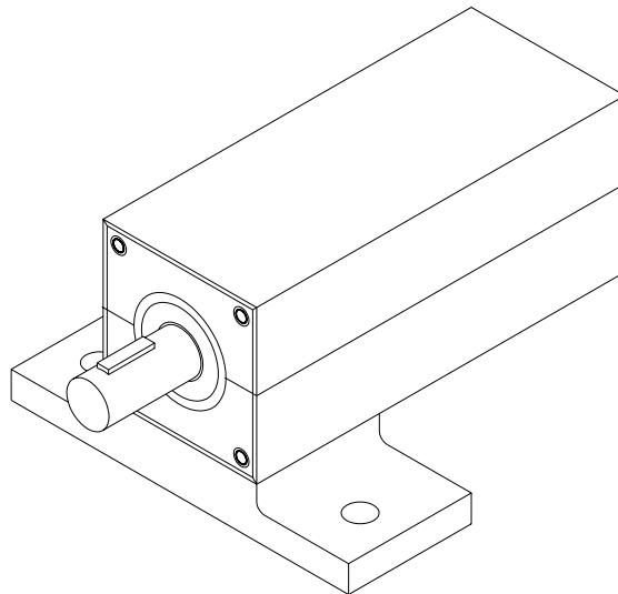
Figure 2.1 TR-1 Resolver Unit
