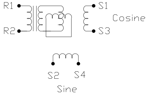
Figure 2.2 TR-1 Electrical Schematic
